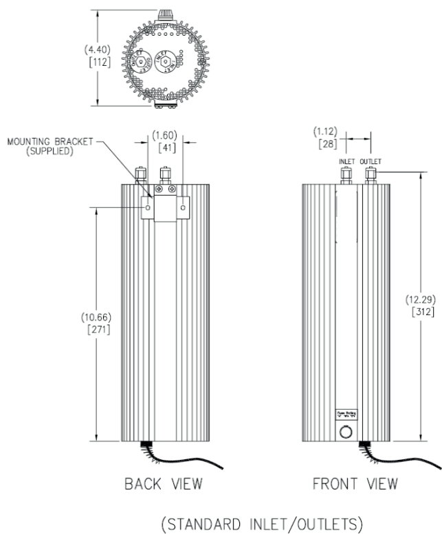
Overall and fixing dimensions - standard
