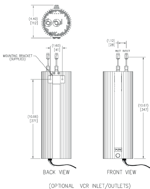
Overall and fixing dimensions - VCR
