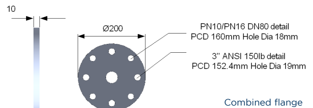
Combined flange
